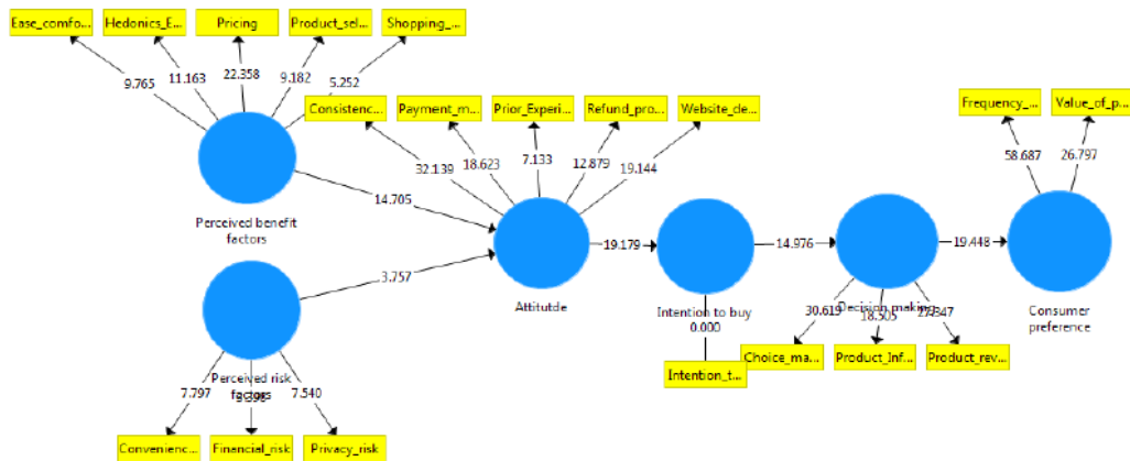
Figure 3: Evaluating Structural Model
