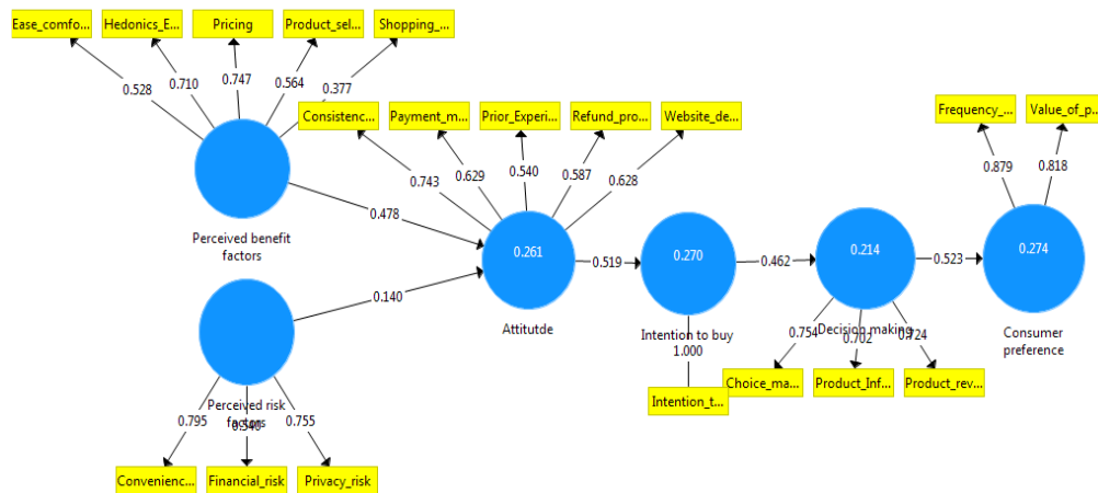
Figure 2: Evaluation of Measurement Model
